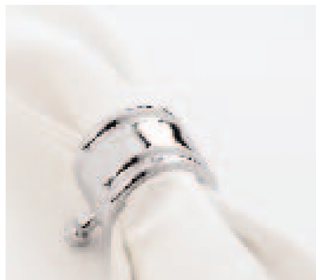
9250 Napkin Ring
