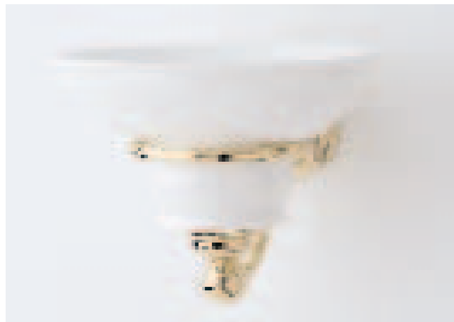
6928 Soap Tray
